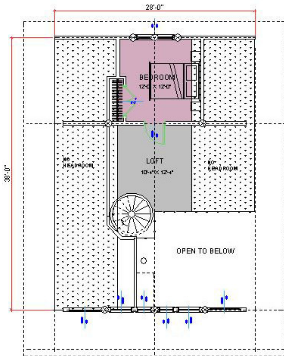
SECOND FLOOR PLAN AREA: 244 SQ. FT.
