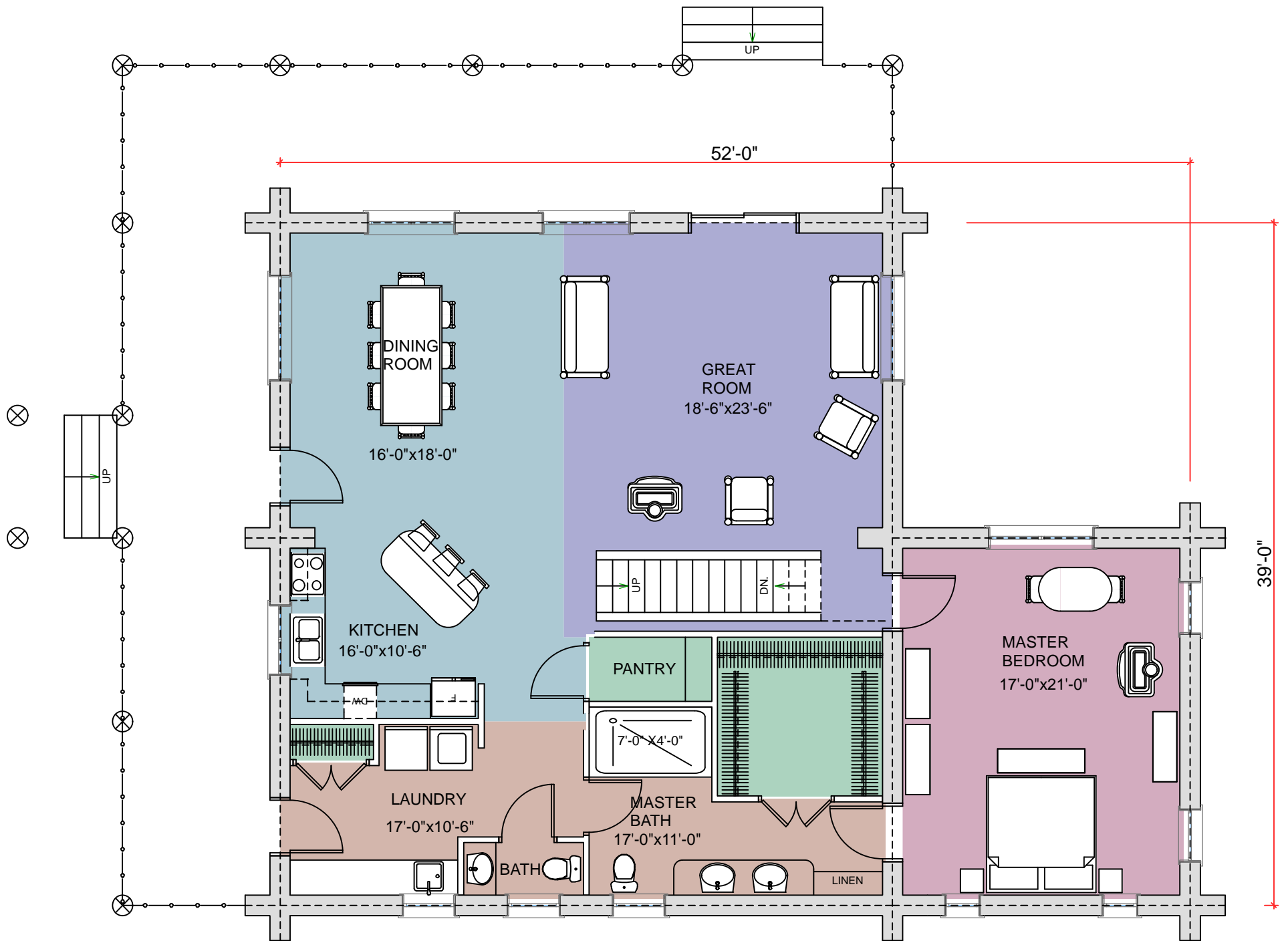
FIRST FLOOR PLAN AREA: 1768 SQ.FT.
